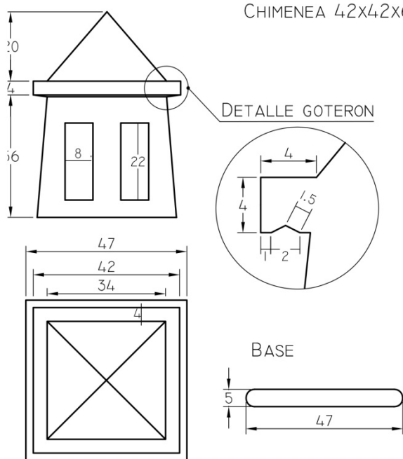
CHIMENEA 42x42x60
